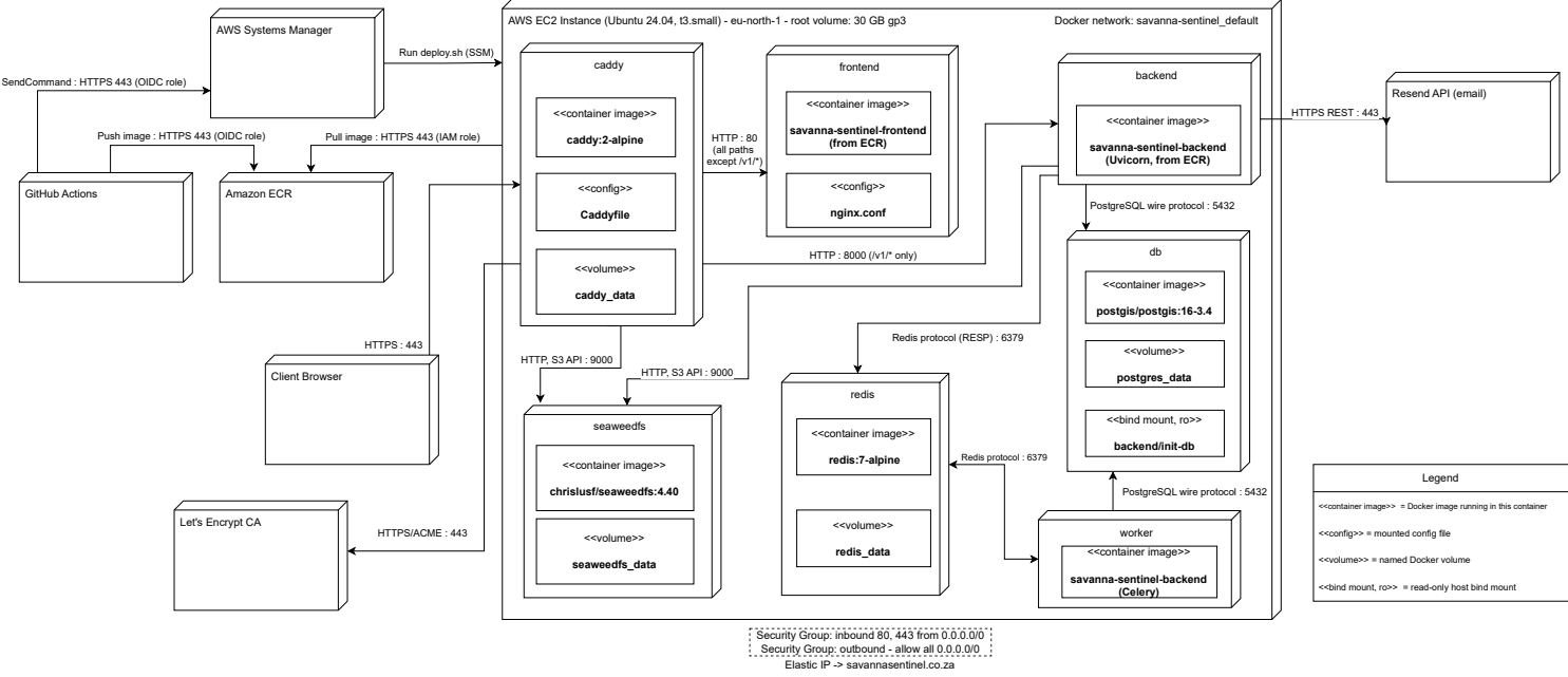
Deployment Diagram - Production Environment (AWS EC2, docker compose --profile prod)
